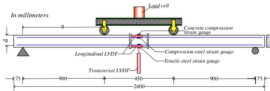
Fig. 3. Experimental set-up
