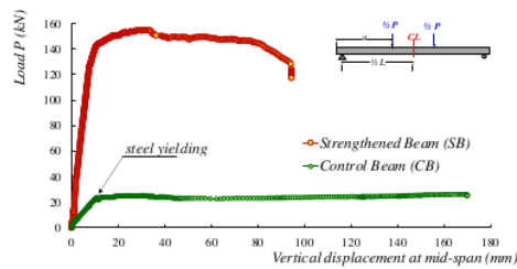
Fig. 4. Load-displacement responses of CB and SB
