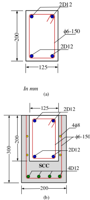
Figs. 1. Details of (a) CB and (b) SB
